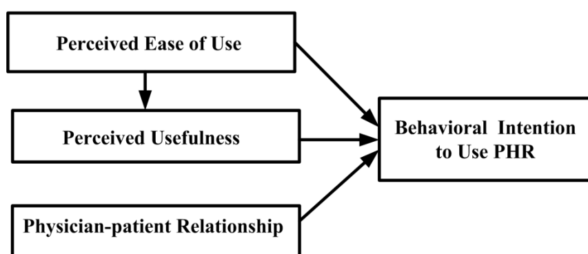
Figure 2. Research model.
